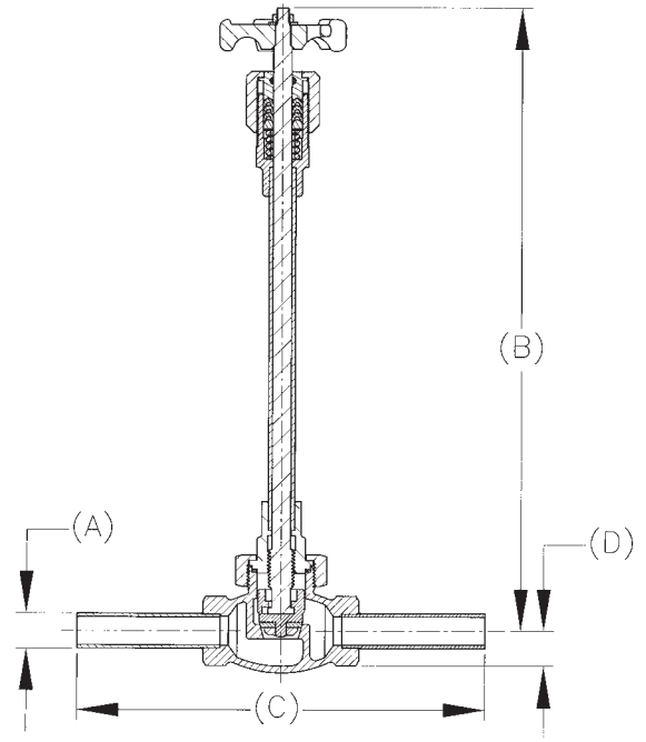
Straight Globe Valve with Stubs
