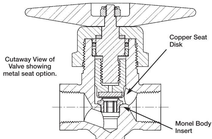
PANEL MOUNT VALVE
