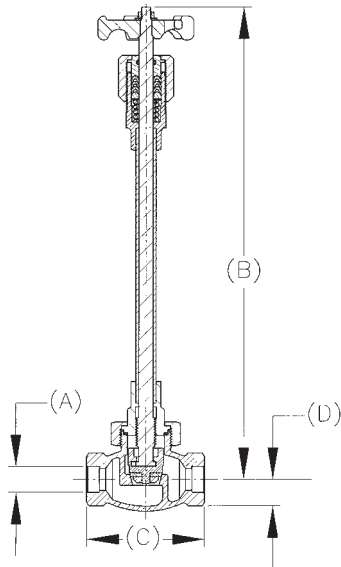
Straight Globe Valve
