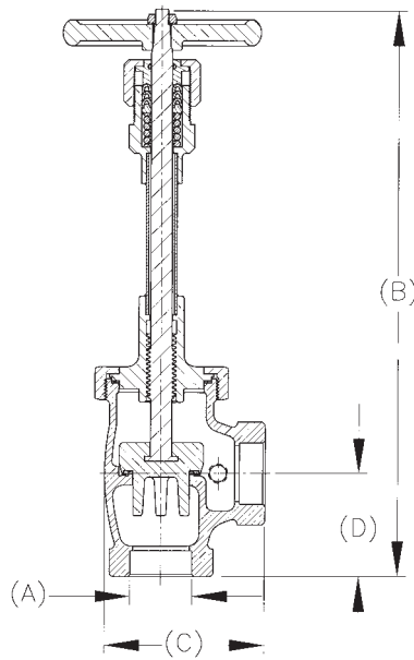
Angle Globe Valve
